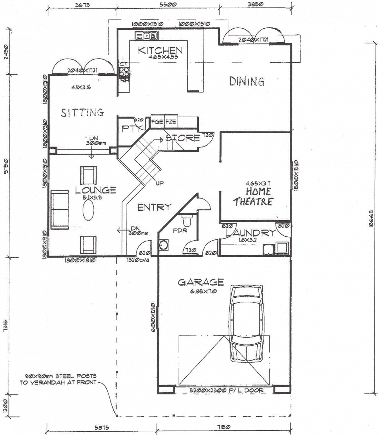
LOWER FLOOR PLAN 1:100
